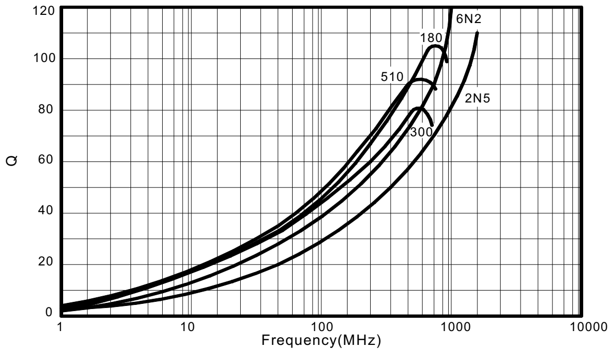
TYPICAL Q vs FREQUENCY
