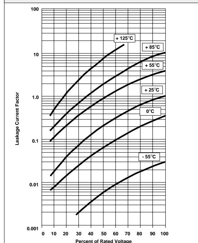
TYPICAL LEAKAGE CURRENT FACTOR RANGE
